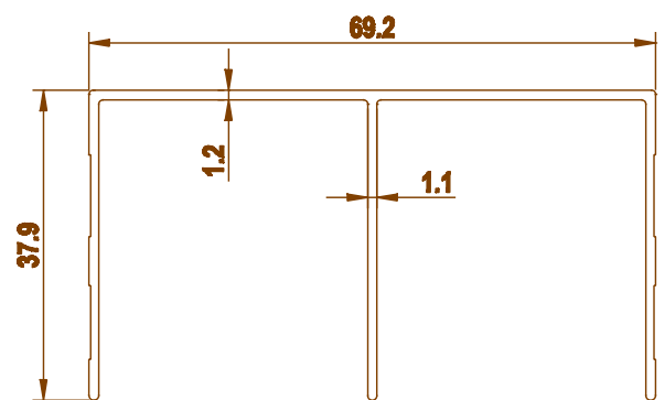
3514 0.551 kg/m
