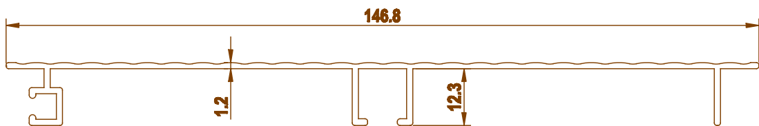
3294 0.623 kg/m
