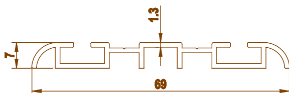
3709 0.440 kg/m
