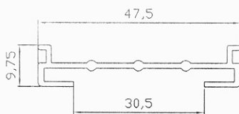
1321 0.304 kg/mt
