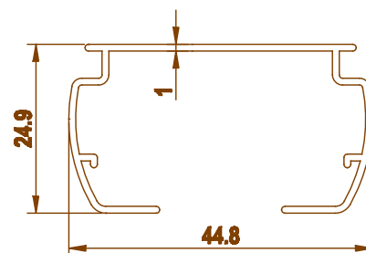
G178 0.323 kg/m
