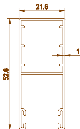
G179 0.455 kg/m
