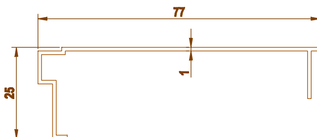
1566 0.330 kg/m
