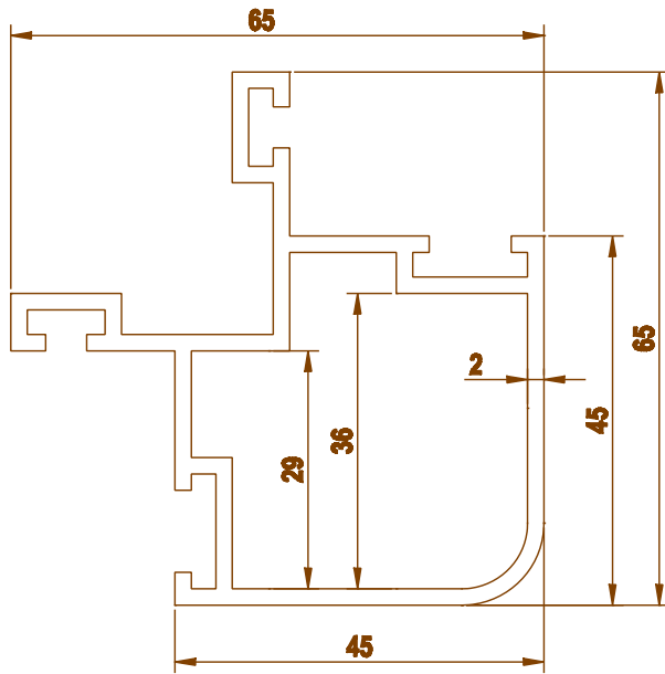
1862 1.377 kg/m
