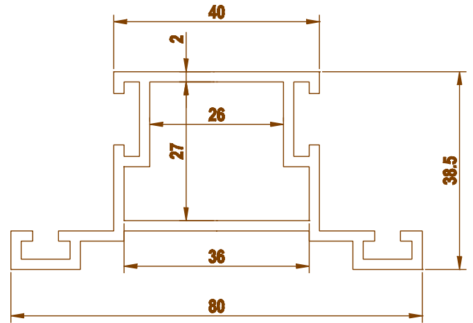
1865 1.231 kg/m
